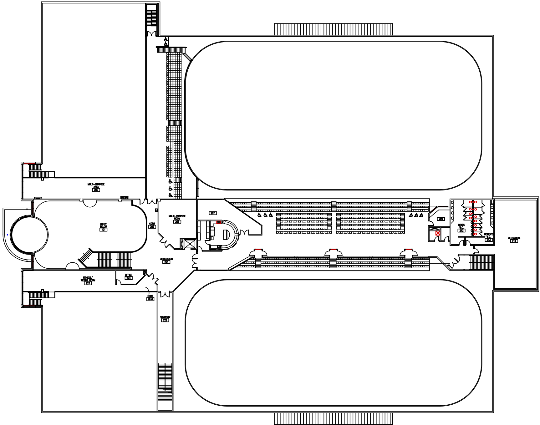
Multi-Plex Upper Floor Plan Scale = 1:500
