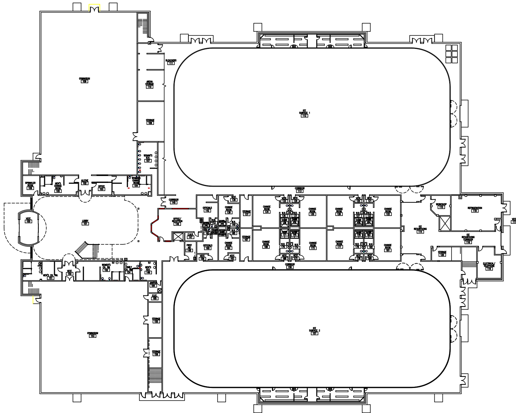
Multi-Plex Lower Floor Plan Scale = 1:500
